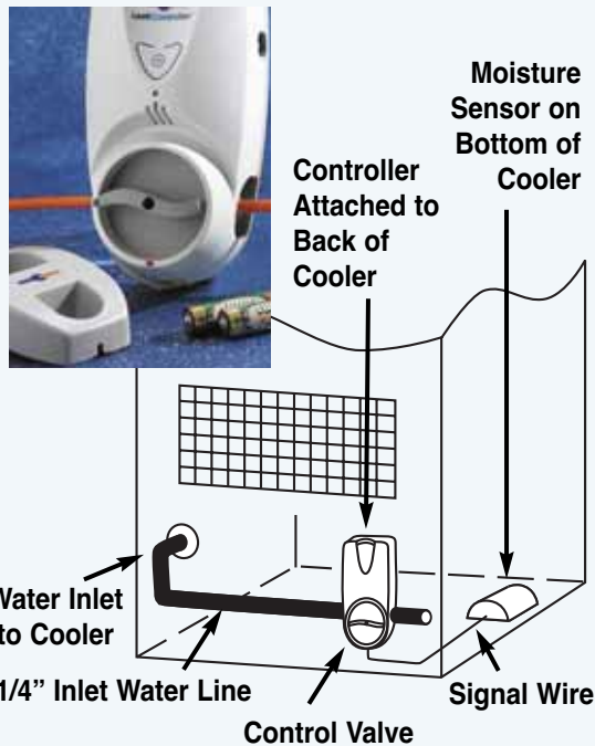
Leak Detector/Installation
